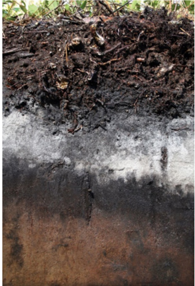
Figure 57.—A wet Spodosol with a splotchy gray and black eluvial horizon above a reddish brown spodic horizon.
