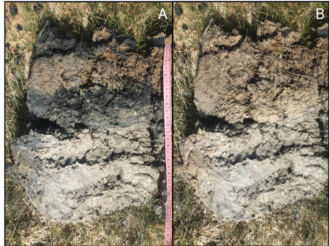
Figure 21.—Indicator A18, Iron Monosulfide in loamy/clayey material. This soil has concentrations of black-colored iron monosulfide (FeS) in the upper 25 cm under moist to wet conditions (A). Concentrations of FeS were confirmed in this soil via the application of dilute (3%) hydrogen peroxide to induce rapid oxidation, resulting in a distinct color change (i.e., an increase in Munsell value of 1 or more) (B).
