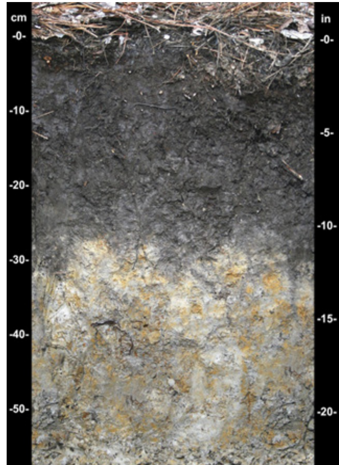
Figure 16.—Indicator A11, Depleted Below Dark Surface. This soil has a thick, dark surface horizon that meets the requirements of indicator A11. Unlike the soil profile in fig. 15, which has a depleted matrix starting around 8 cm below the dark surface horizon, this soil has a depleted matrix that starts at a depth of about 29 cm, which is too deep to meet the requirements of indicator F3, Depleted Matrix. Indicator A11 allows a deeper depleted matrix than indicator F3.
