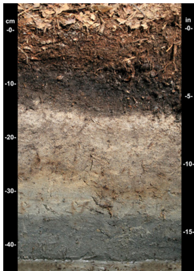
Figure 2.— The soil profile above consists of an 8 cm layer of peat and/or mucky peat underlain by a 1 cm layer of muck. The remaining soil layers are sandy soil material. In LRRs R, W, X, and Y, observations would begin below the peat, mucky peat, and muck layers (9 cm). When using Indicators S2 or S3 observations would start at the actual soil surface. In all remaining LRRs, observations would begin at the muck surface (8 cm).
