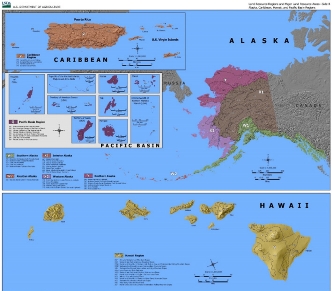
Figure 7.—Map of USDA land resource regions and major land resource areas in the nonconterminous United States.
