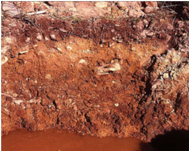
Figure 41.—Indicator F21, Red Parent Material. This indicator should be used only in areas of red parent material that are resistant to reduction. Not all red soils formed in red parent material.
