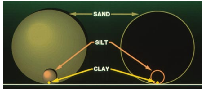
Figure 24.—The relative sizes of sand, silt, and clay.
