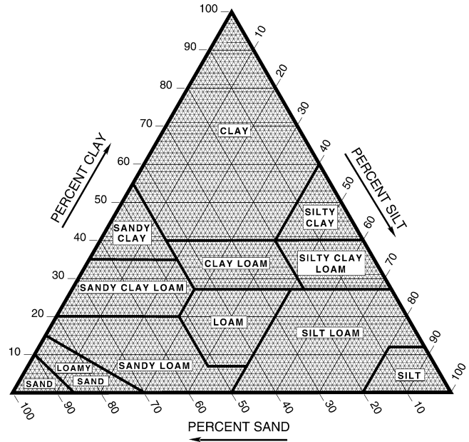
Figure 23.—USDA soil texture classes.
